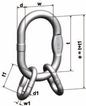
VWI Master link assembly
