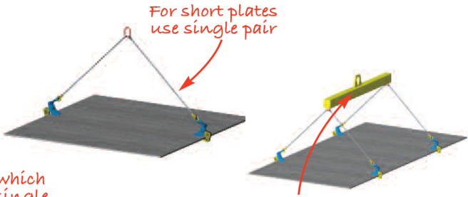
For long plates use spreader beam
